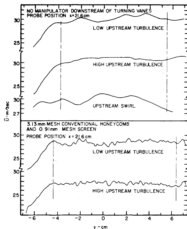
Fig. 3 Lateral profiles of mean velocity with either a conventional honeycomb or no flow manipulator downstream of turning vanes in several flow conditions.
