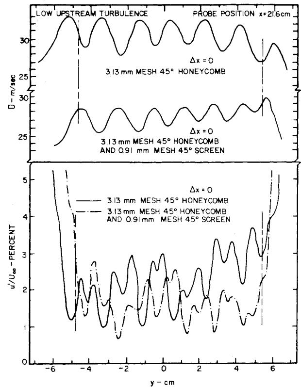
Fig. 5 Lateral profiles of mean velocity and turbulence intensity with a 3.13 mm mesh 45 deg honeycomb positioned at trailing edges of turning vanes with and without a 0.91 mm mesh 45 deg screen at downstream end of honeycomb in low turbulence flow condition.
