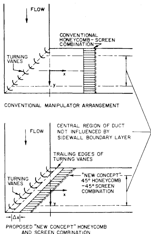
Fig. 1 Schematic of proposed new-concept 45 deg honeycomb and comparison with a conventional honeycomb.
