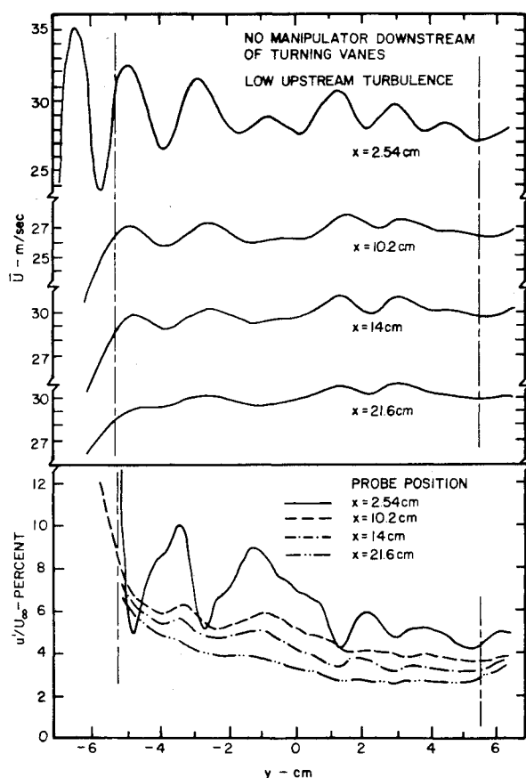
Fig. 2 Lateral profiles of mean velocity and turbulence intensity at several distances downstream of turning vanes with low upstream turbulence.
