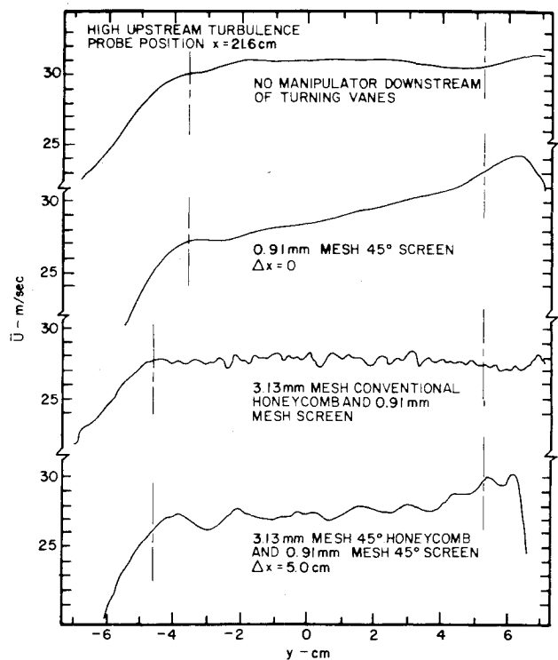
Fig. 11 Effect of using no manipulator, a 45 deg screen, a conventional honeycomb-screen combination, and a 45 deg honeycomb-45 deg screen combination downstream of turning vanes on lateral profile of mean velocity in high turbulence flow condition.
