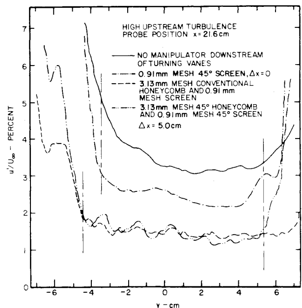
Fig. 12 Effect of using no manipulator, a 45 deg screen, a conventional honeycomb-screen combination, and a 45 deg honeycomb-45 deg screen combination downstream of turning vanes on lateral profile of turbulence intensity in high turbulence flow condition.
