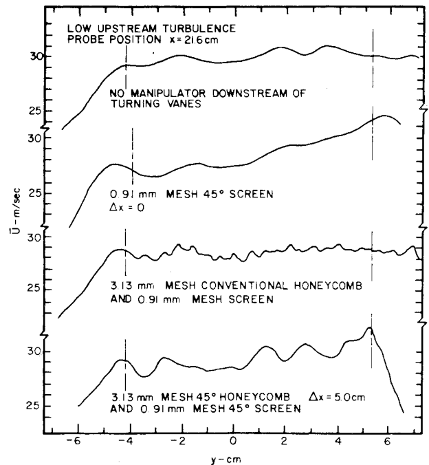
Fig. 9 Effect of using no manipulator, a 45 deg screen, a conventional honeycomb-screen combination, and a 45 deg honeycomb-45 deg screen combination downstream of turning vanes on lateral profile of mean velocity in low turbulence flow condition.
