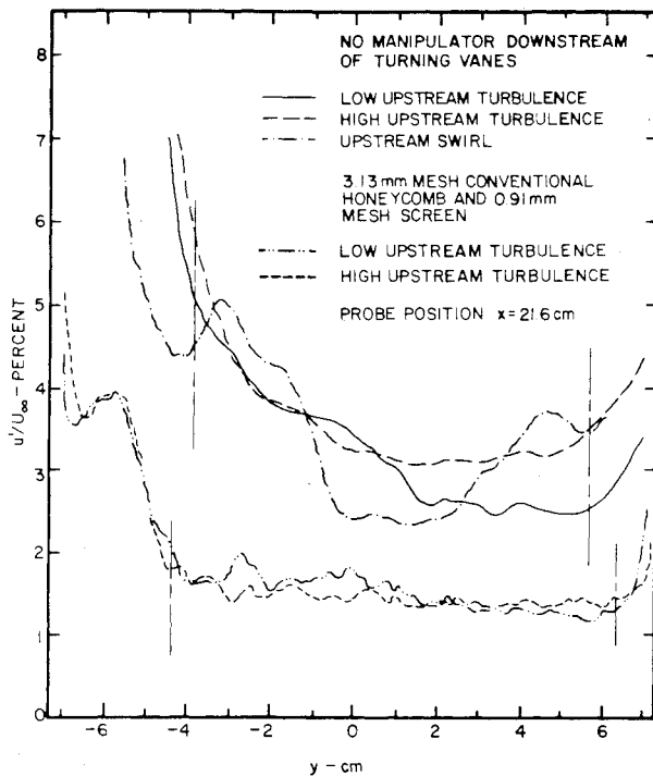
Fig. 4 Lateral profiles of turbulence intensity with either a conventional honeycomb or no flow manipulator downstream of turning vanes in several flow conditions.
