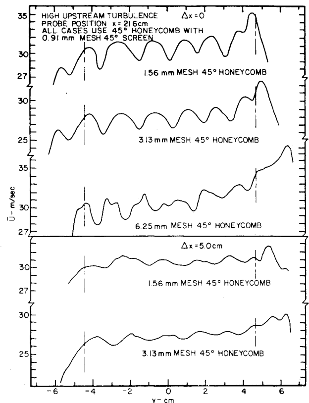
Fig. 7 Effect of 45 deg honeycomb mesh on lateral profiles of mean velocity for a 45 deg honeycomb-45 deg screen combination with no separation from turning vanes, \Delta x = 0 and 5.0 cm in high turbulence flow condition.
