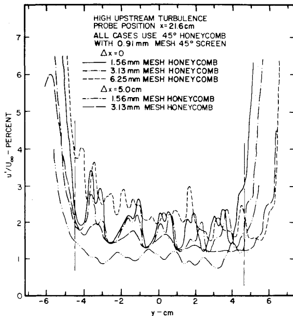
Fig. 8 Effect of 45 deg honeycomb mesh on lateral profiles of turbulence intensity for a 45 deg honeycomb-45 deg screen combination with no separation from turning vanes, \Delta x = 0 and 5.0 cm in high turbulence test flow condition.
