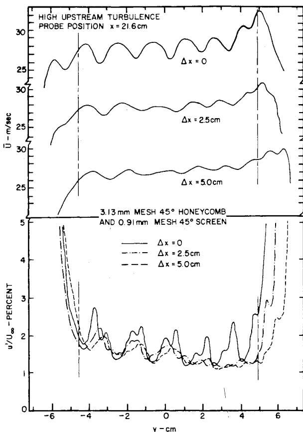
Fig. 6 Effect of separation between 45 deg honeycomb-45 deg screen combination and trailing edges of turning vanes on lateral profiles of mean velocity and turbulence intensity in high turbulence flow condition.
