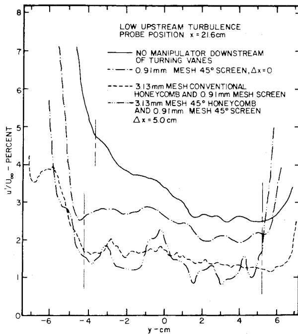
Fig. 10 Effect of using no manipulator, a 45 deg screen, a conventional honeycomb-screen combination, and a 45 deg honeycomb-45 deg screen combination downstream of turning vanes on lateral profile of turbulence intensity in low turbulence flow condition.
